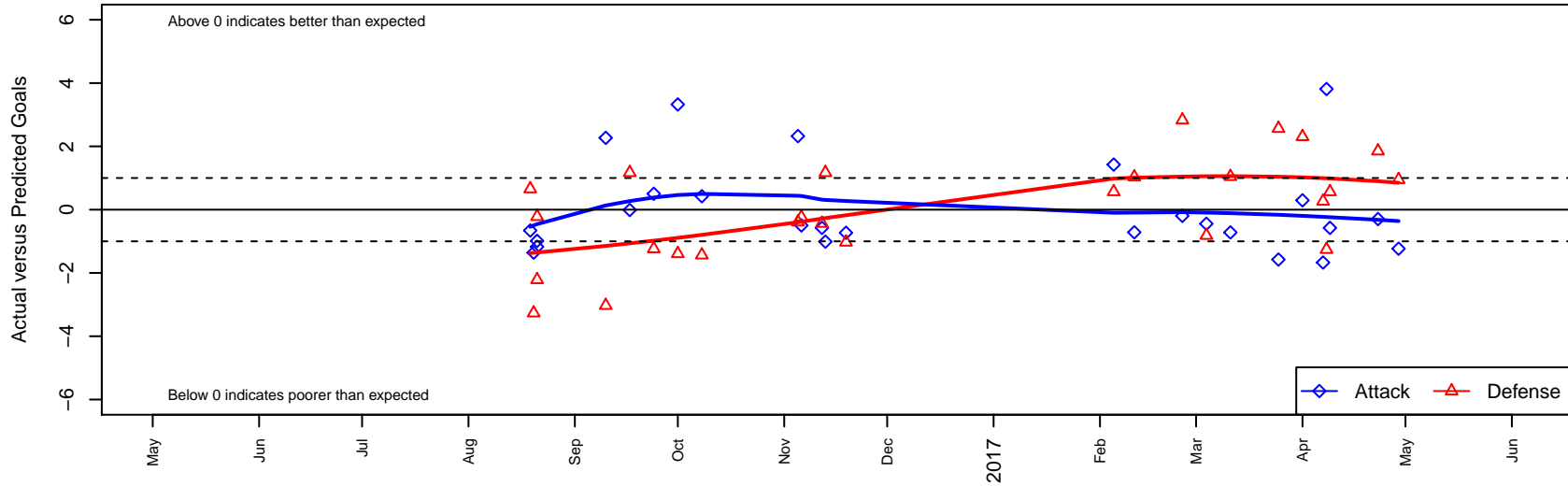
NPSA Titans Navy Mercer Island B06 Dots are actual minus expected GF (blue circles) and GA (red triangles). Blue line is smoothed change in attack strength. Red is smoothed change in defense strength.
